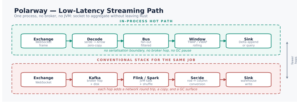
Figure 3: The same job expressed two ways. Every box in the lower path is a process boundary: a serialisation, a network round trip, and a garbage collector that may pause at the wrong moment.
