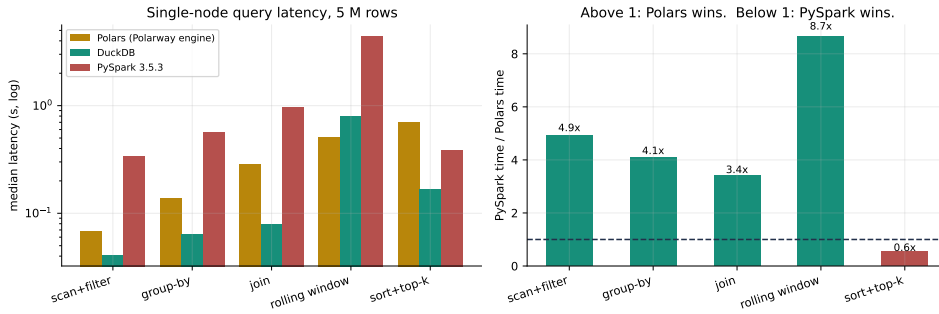
Figure 6: Left: median latency per query (log scale). Right: the PySpark-to-Polars ratio, with the break-even line marked. The sort+top- k bar falls below it — PySpark wins that query.
