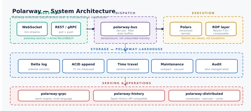
Figure 1: Polarway system architecture. Ingestion materialises network sources directly into Arrow; the bus fans batches out in-process; execution pairs the Polars kernels with the Railway-Oriented error layer; and every stage exchanges versioned tables with the Delta-backed storage layer.
