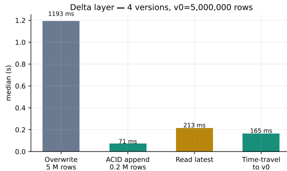
Figure 2: Delta layer operation costs. The append path writes only new files and one log entry, which is why it is an order of magnitude cheaper than the overwrite.
