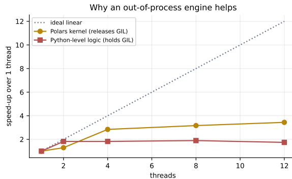
Figure 5: Thread scaling for GIL-releasing and GIL-holding work. Polars already releases the GIL inside its kernels, so threads do help — but only to about 3.4\times on twelve cores. Python-level logic plateaus near 1.8\times .
