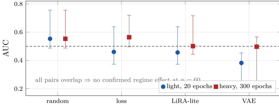
Figure 9: Compiled-probe AUCs with 95% block-bootstrap intervals. The heavy regime trends above the light regime for loss , lira and vae , as theory predicts — but every interval pair overlaps, so by the claim discipline of §5.1 the trend is reported as a trend, not as a result.
