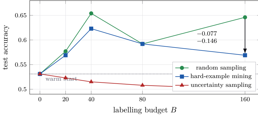
Figure 11: Neither active-learning heuristic beat random sampling at any budget. At the largest budget the deficits are -0.077 (hard-example mining) and -0.146 (uncertainty sampling). Uncertainty sampling never improves on the warm start at all.
