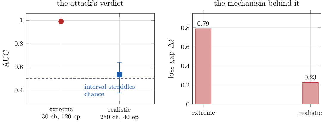
Figure 8: The same attack in two regimes. Left: the extreme regime is significant, the realistic regime is not distinguishable from chance. Right: the loss gap collapses by 71% — from +0.790 to +0.226 — purely from 8.3\times more data and 3\times fewer epochs.
