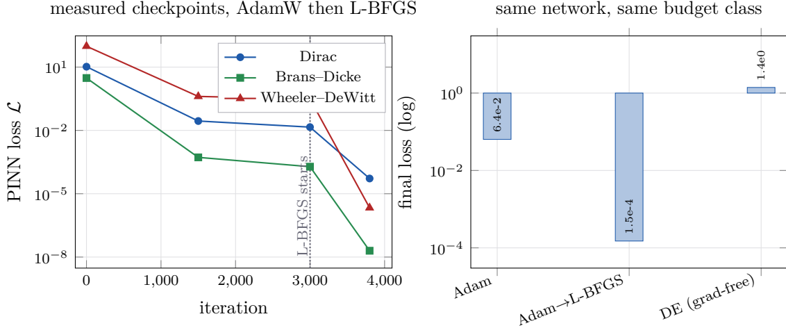
Figure 4: Left: measured loss checkpoints for the three full-size problems. The AdamW stage runs 3000 iterations and the L-BFGS stage 800; the near-vertical segment after the dotted line is the quasi-Newton contribution. Right: the 206-parameter ablation of Table 2 on a log scale.
