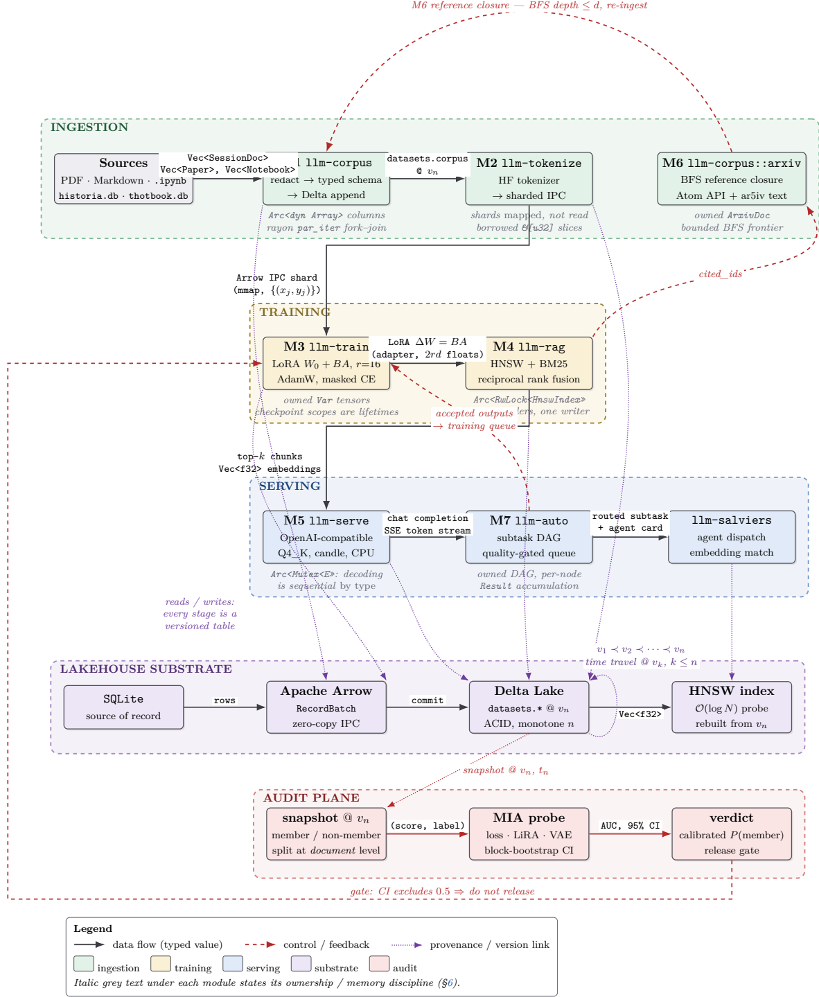
Figure 1: ThotBook-AI end to end. Solid edges carry typed values; dashed edges carry control and feedback; dotted edges bind a stage to the lakehouse version it reads or writes. The substrate row is not storage beneath the pipeline but part of it: each stage’s input is a table at a numbered version v_k , which is what makes both time travel and the audit plane possible. The audit plane (red) reads a snapshot at v_n , runs the membership probe of §5.3, and returns a calibrated verdict that gates release.
