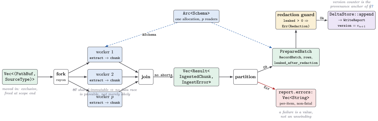
Figure 2: Ownership and error flow inside one stage (M1 ingest). Files are moved into a rayon fork-join; workers hold only shared-immutable borrows, which is why the parallelism needs no lock and no defensive copy. The join produces a Vec<Result<...> , so a per-item failure is an ordinary value that the batch survives — the property that makes the leaked_after_redaction counter total over all rows and therefore trustworthy as a gate. Only a batch that passes the redaction guard reaches DeltaStore::append , which returns the new version v_{n+1} .
