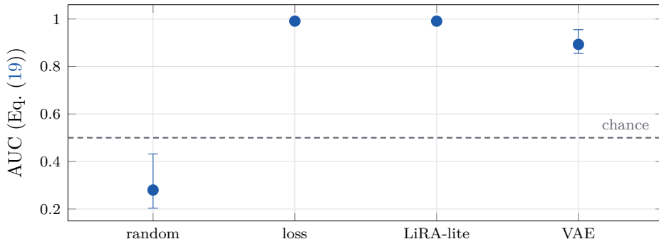
Figure 6: Attack AUC with 95% block-bootstrap intervals, extreme regime. The random control’s interval sits below chance rather than on it — an n = 30 artefact, discussed in Remark 5.5 — while the three real attacks’ intervals are far above and mutually overlapping, so no ordering among them is claimed.
