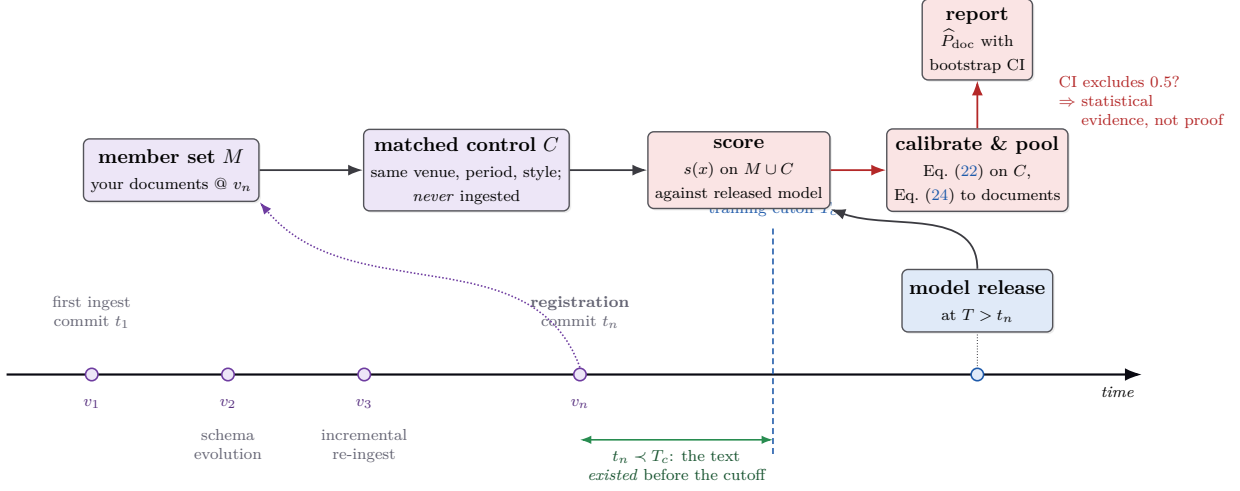
Figure 12: The provenance protocol on a time axis. Corpus versions v_1 \prec \dots \prec v_n are lakehouse commits with timestamps; registration at (v_n, t_n) must precede the target model’s training cutoff T_c . The audit plane (red, matching Figure 1) scores the member set and a matched control against the released model, calibrates on the control, and pools to a document-level probability with an interval.
