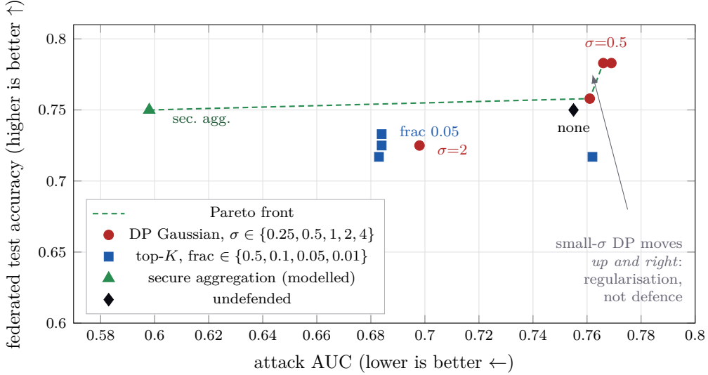
Figure 10: Privacy/utility Pareto frontier over all eleven measured configurations of Table 15. The frontier (green dashed) consists of exactly three points: secure aggregation, which cuts the attack by 0.157 at zero accuracy cost, and the two small-noise DP settings, which improve accuracy. Every top- K configuration and every large- \sigma DP configuration is dominated by secure aggregation.
