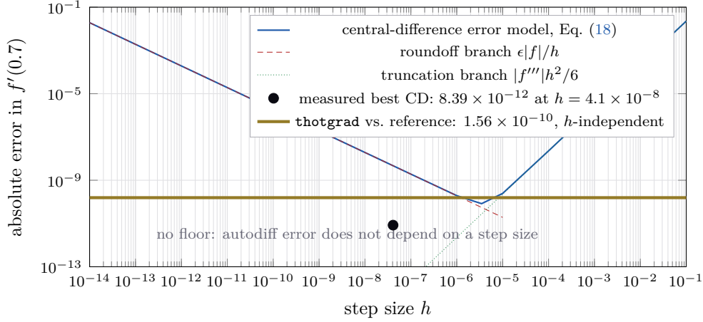
Figure 3: The finite-difference error floor and its absence for automatic differentiation. The V-shaped curve is the analytic model of Eq. (18) evaluated for the probe network ( |f'''|/6 \approx 2.27 , \epsilon_{\text{mach}}|f| \approx 1.92 \times 10^{-16} ), with its two asymptotic branches. The horizontal line is thotgrad ’s discrepancy against the reference derivative: it is a single number, not a function of h , because no step size is involved.
