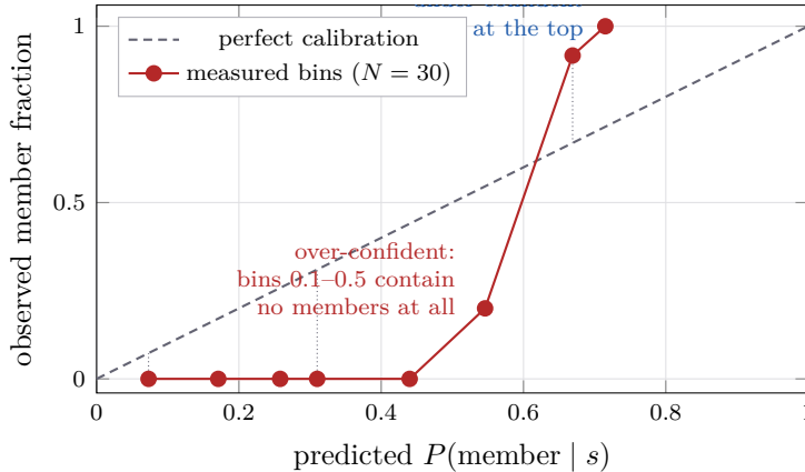
Figure 7: Reliability diagram for Eq. (22), measured bins. \text{ECE} = 0.2565 . The low-confidence bins are over-confident — every prediction between 0.073 and 0.440 is a non-member — and the 0.669 bin is under-confident, containing 91.7% members. Bin populations are in Table 8.
